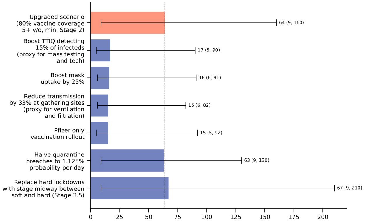
Panel A: Daily infections
